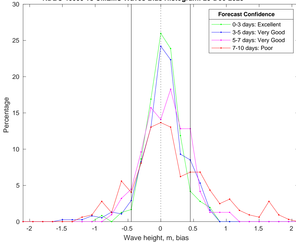
NDBC 46059 vs CMEMS Waves Bias Histogram: 25-Dec-2025
