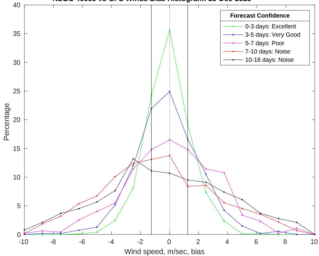
NDBC 46059 vs GFS Winds Bias Histogram: 25-Dec-2025
