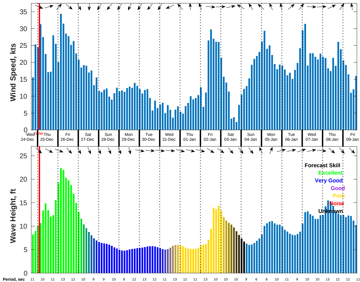
Wind & Wave Forecast for NDBC 46059 from 24-Dec-2025 17:00:00 to 09-Jan-2026 17:00:00
