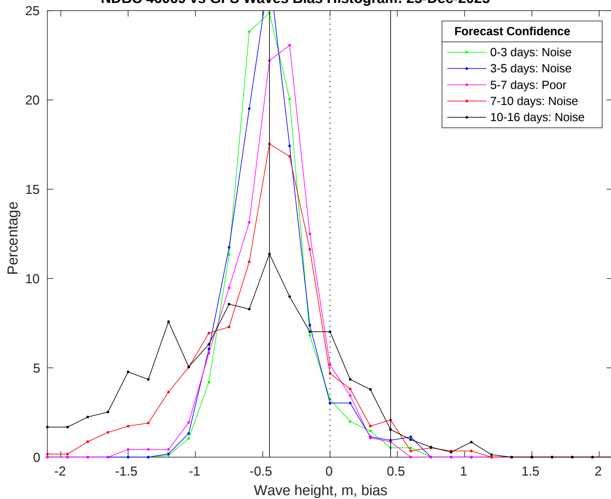
NDBC 46069 vs GFS Waves Bias Histogram: 25-Dec-2025
