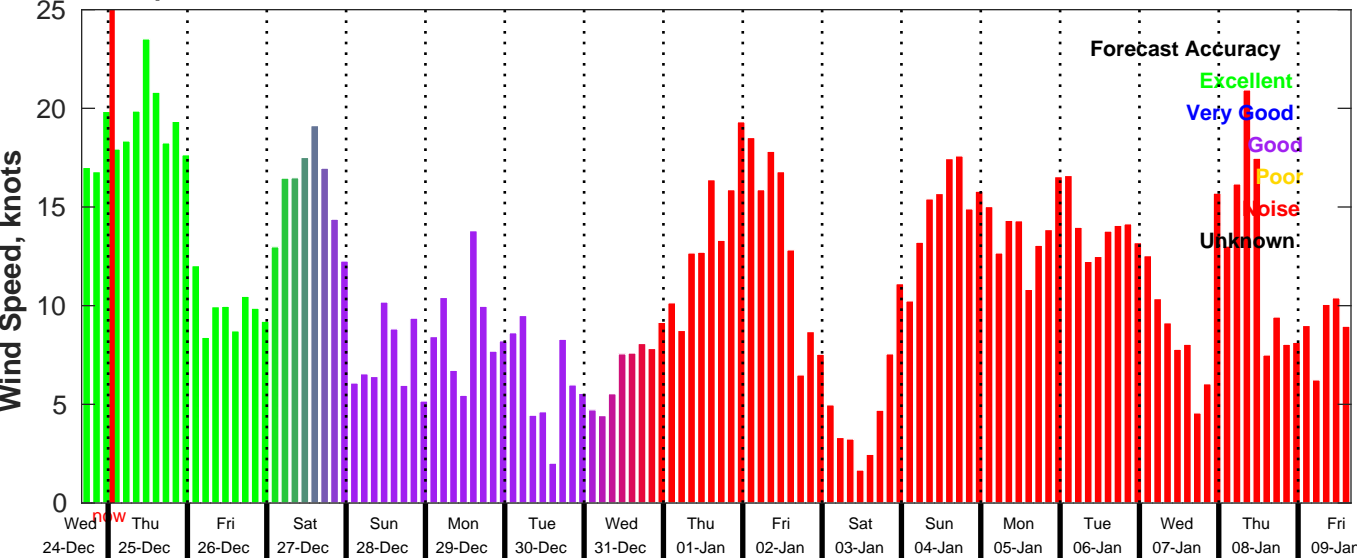
GFS Wind Speed Forecast for NDBC 46069 from 24-Dec-2025 16:00:00 to 09-Jan-2026 16:00:00
