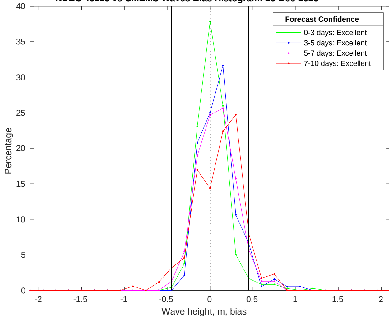
NDBC 46215 vs CMEMS Waves Bias Histogram: 25-Dec-2025
