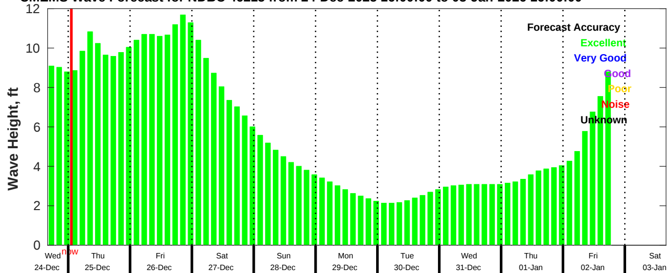
CMEMS Wave Forecast for NDBC 46215 from 24-Dec-2025 16:00:00 to 03-Jan-2026 16:00:00
