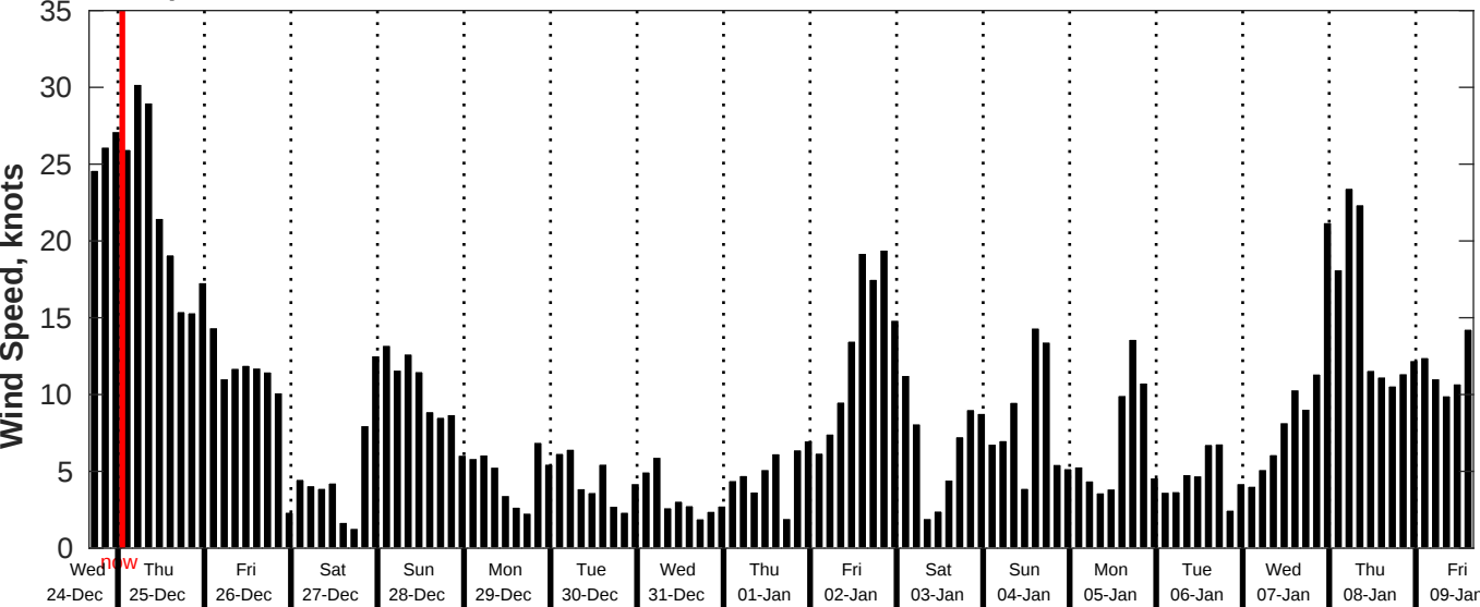
GFS Wind Speed Forecast for NDBC 46215 from 24-Dec-2025 16:00:00 to 09-Jan-2026 16:00:00
