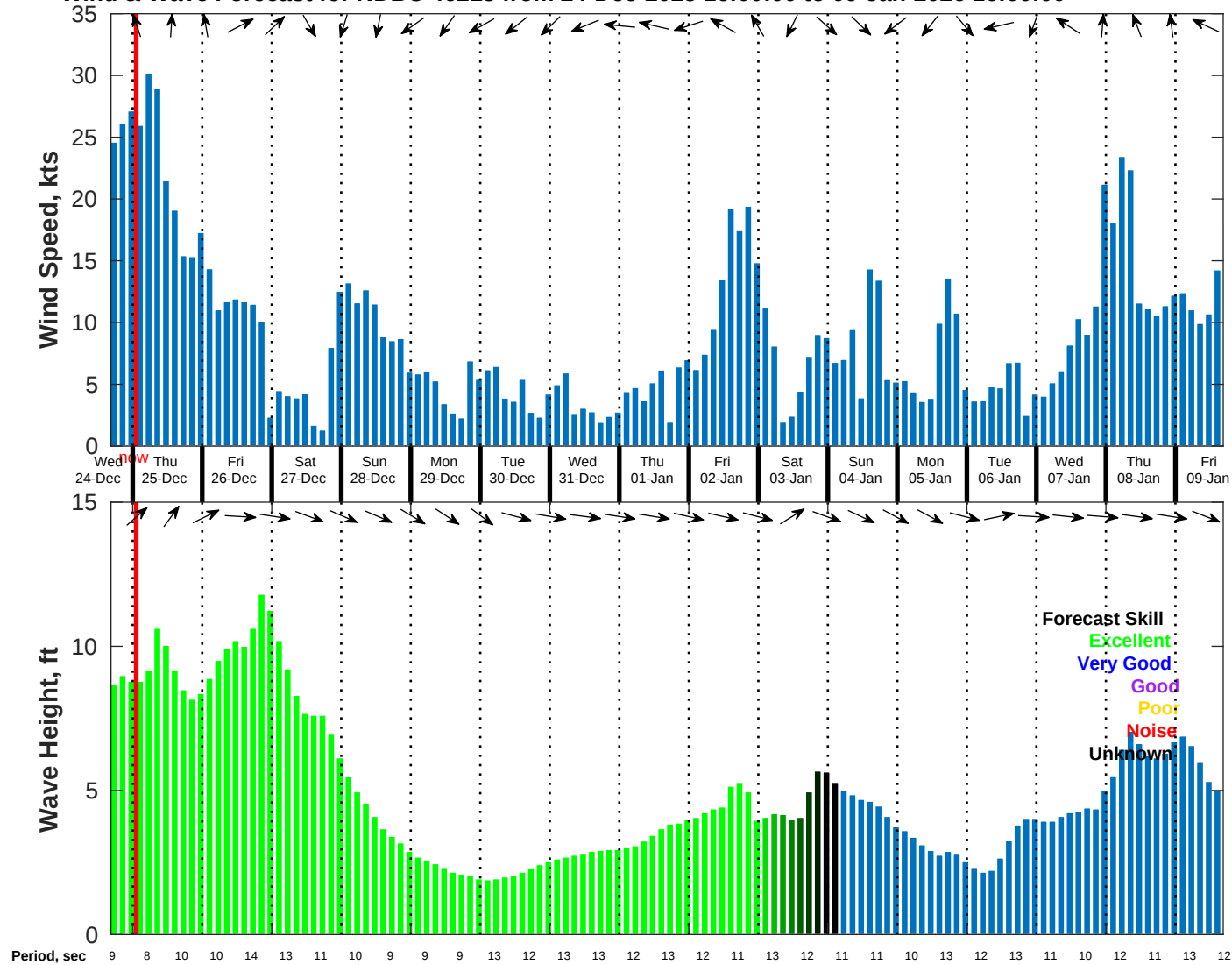
Wind & Wave Forecast for NDBC 46215 from 24-Dec-2025 16:00:00 to 09-Jan-2026 16:00:00
