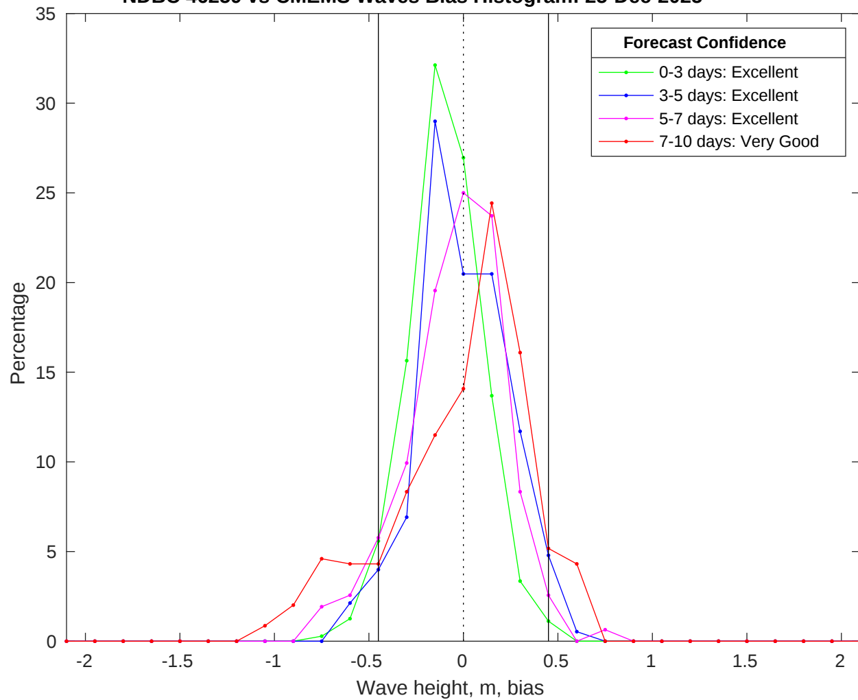
NDBC 46259 vs CMEMS Waves Bias Histogram: 25-Dec-2025
