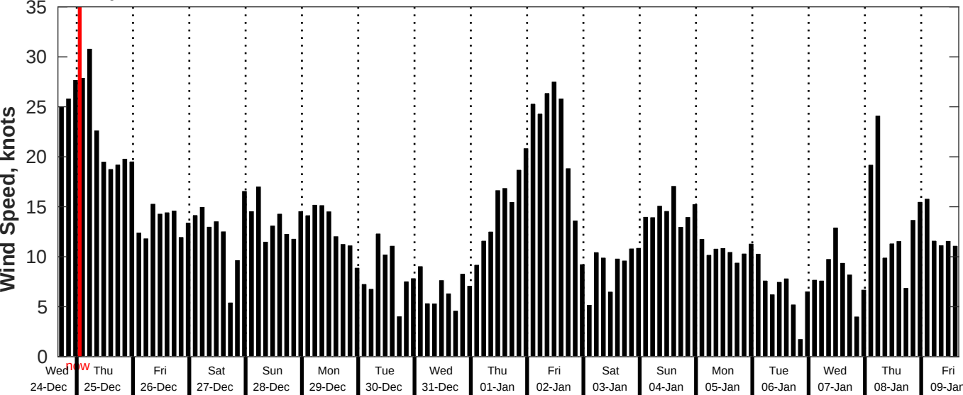
GFS Wind Speed Forecast for NDBC 46259 from 24-Dec-2025 16:00:00 to 09-Jan-2026 16:00:00
