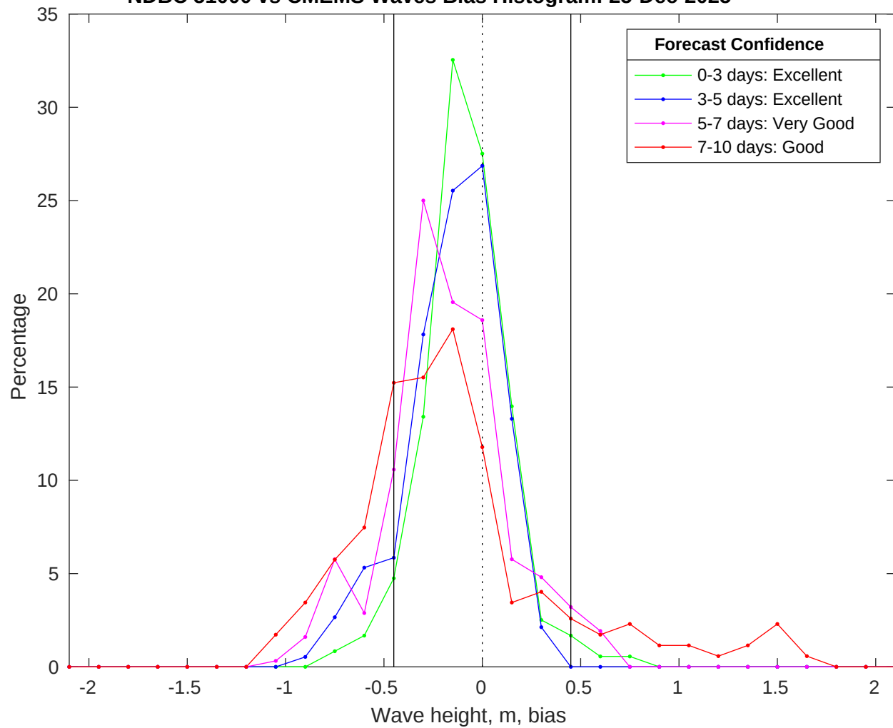
NDBC 51000 vs CMEMS Waves Bias Histogram: 25-Dec-2025
