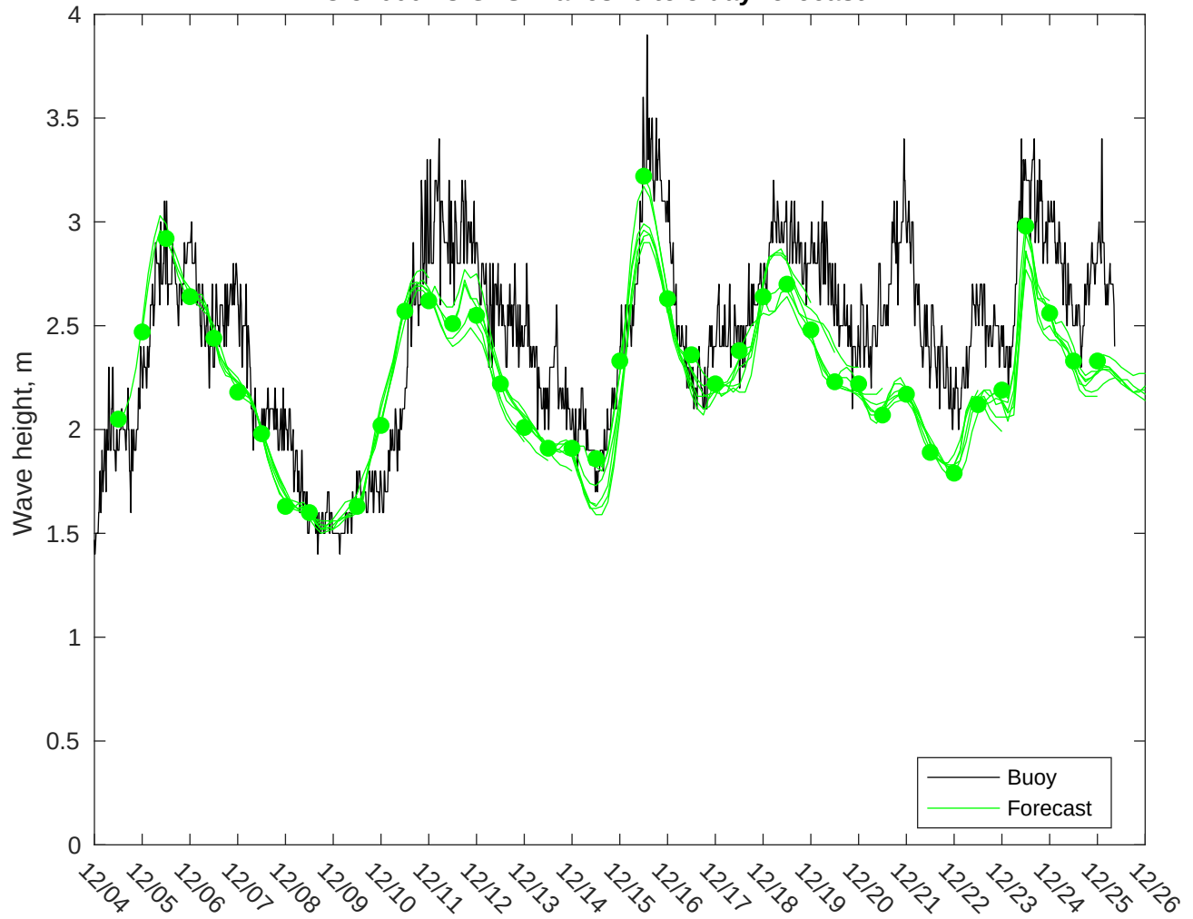
NDBC 51000 vs GFS Waves: 0 to 3 day forecast
