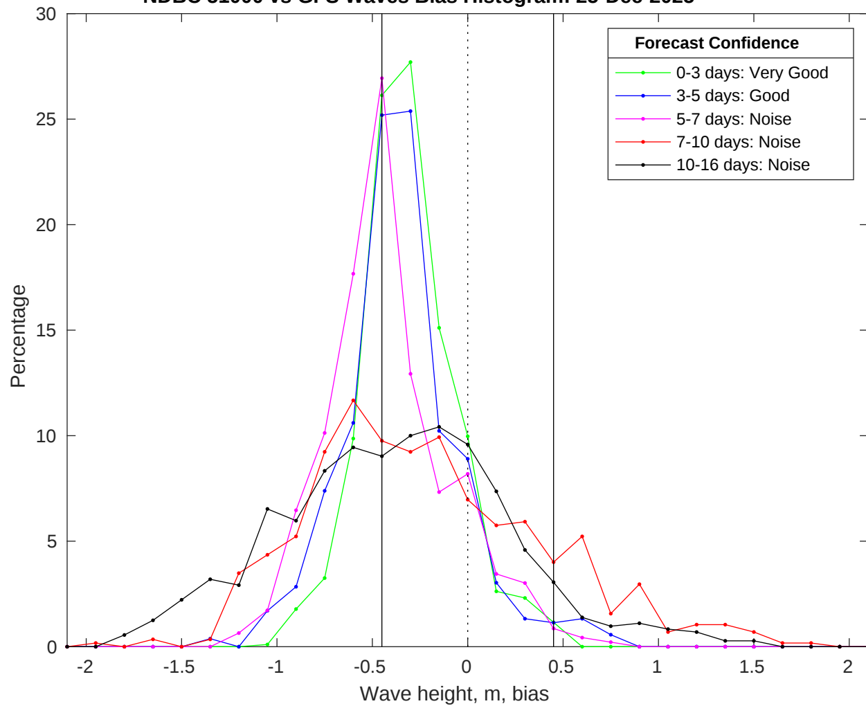
NDBC 51000 vs GFS Waves Bias Histogram: 25-Dec-2025
