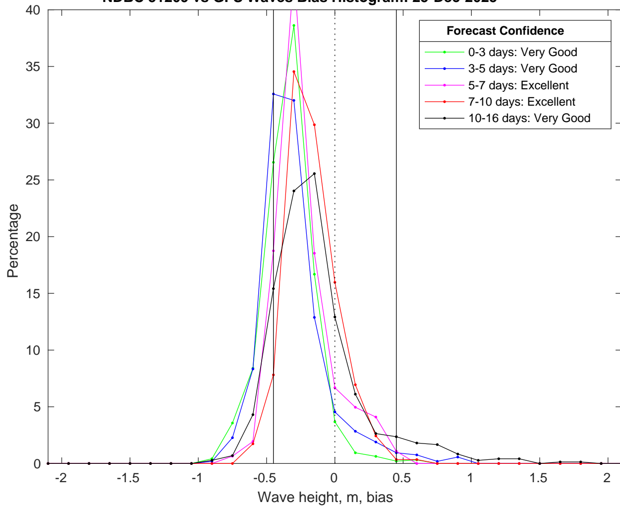
NDBC 51209 vs GFS Waves Bias Histogram: 25-Dec-2025
