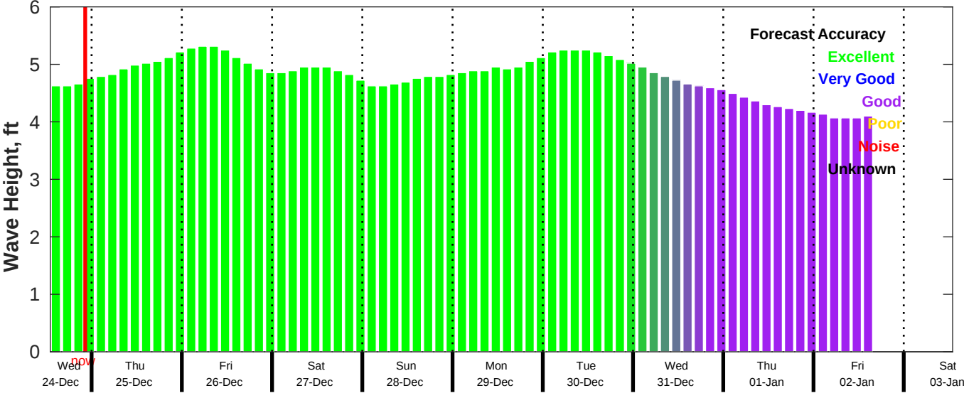
CMEMS Wave Forecast for NDBC 51209 from 24-Dec-2025 13:00:00 to 03-Jan-2026 13:00:00
