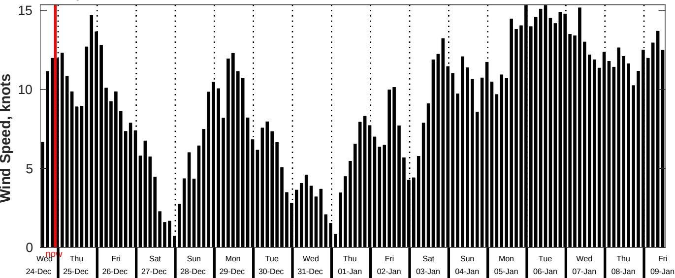
GFS Wind Speed Forecast for NDBC 51209 from 24-Dec-2025 13:00:00 to 09-Jan-2026 13:00:00
