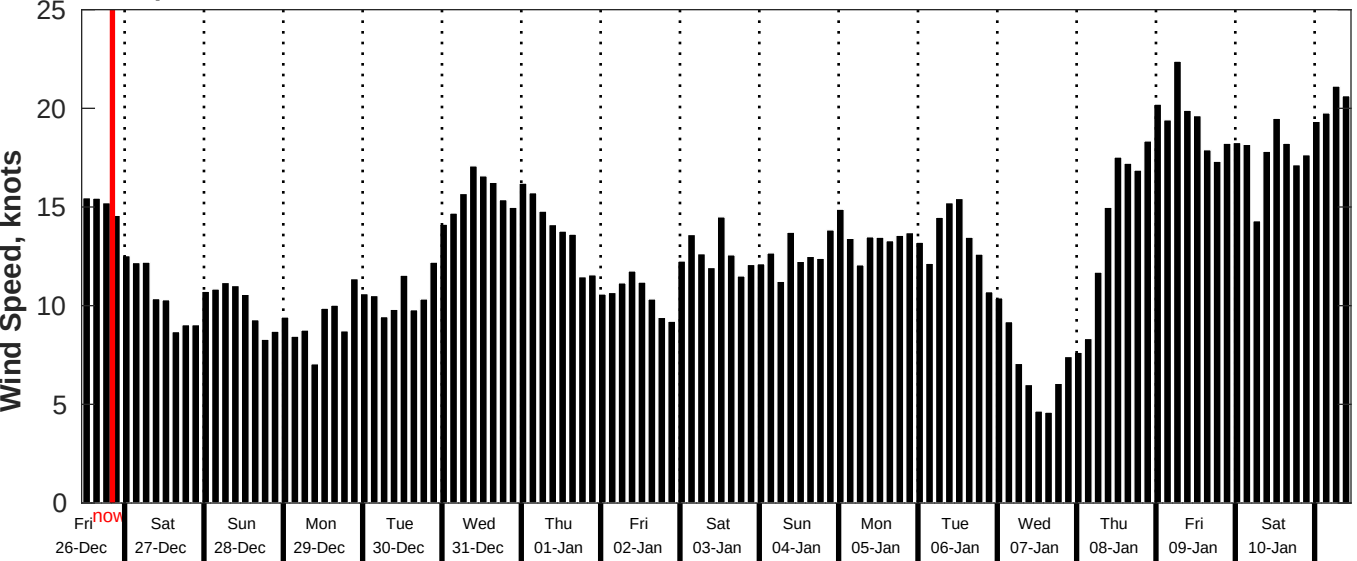
GFS Wind Speed Forecast for NDBC 52211 from 25-Dec-2025 11:00:00 to 10-Jan-2026 11:00:00
