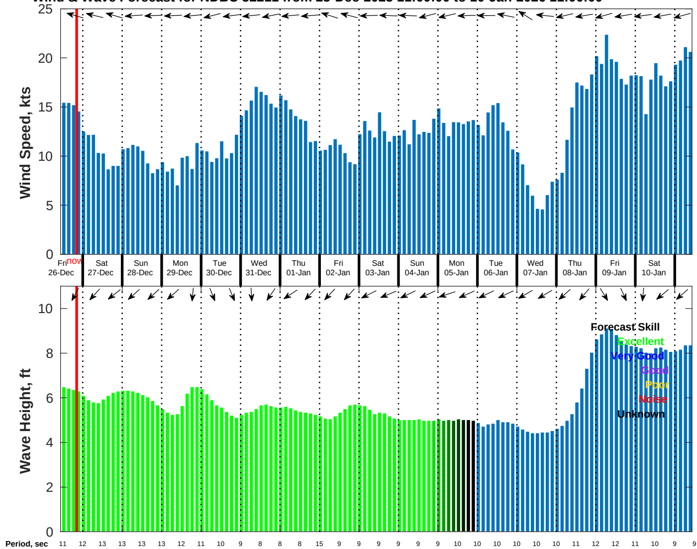
Wind & Wave Forecast for NDBC 52211 from 25-Dec-2025 11:00:00 to 10-Jan-2026 11:00:00
