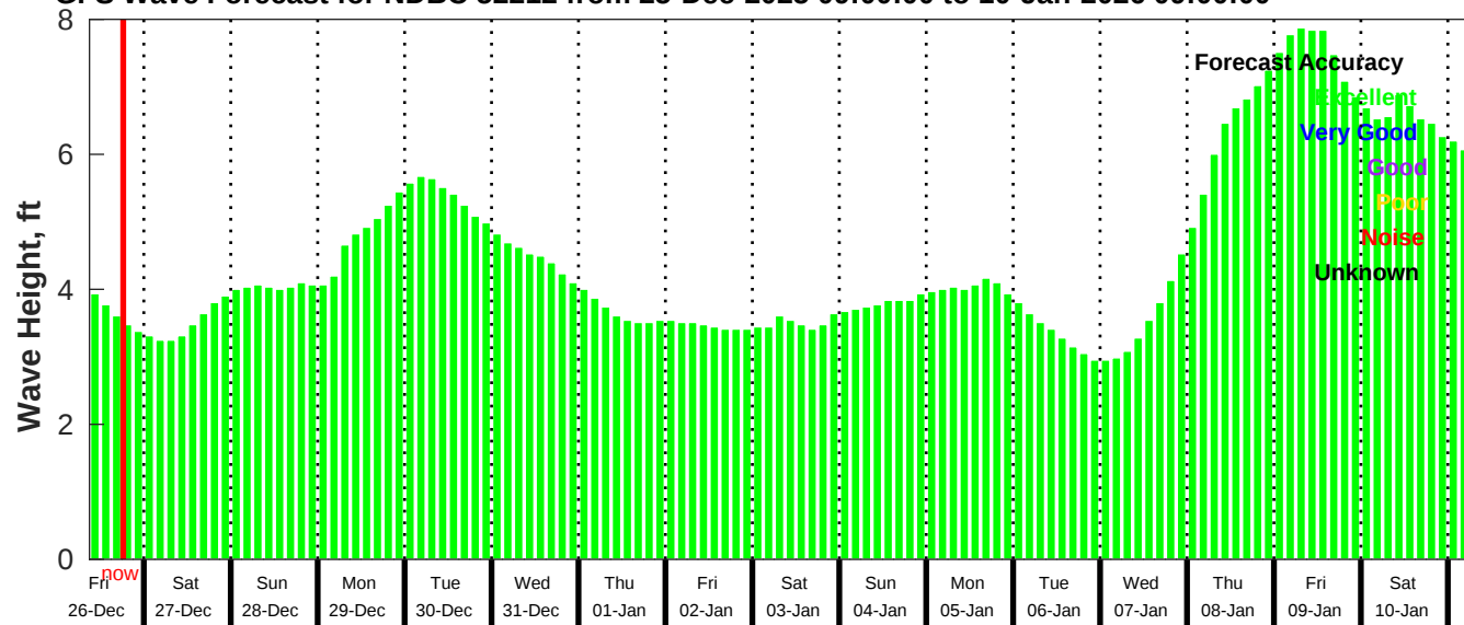
GFS Wave Forecast for NDBC 52212 from 25-Dec-2025 09:00:00 to 10-Jan-2026 09:00:00
