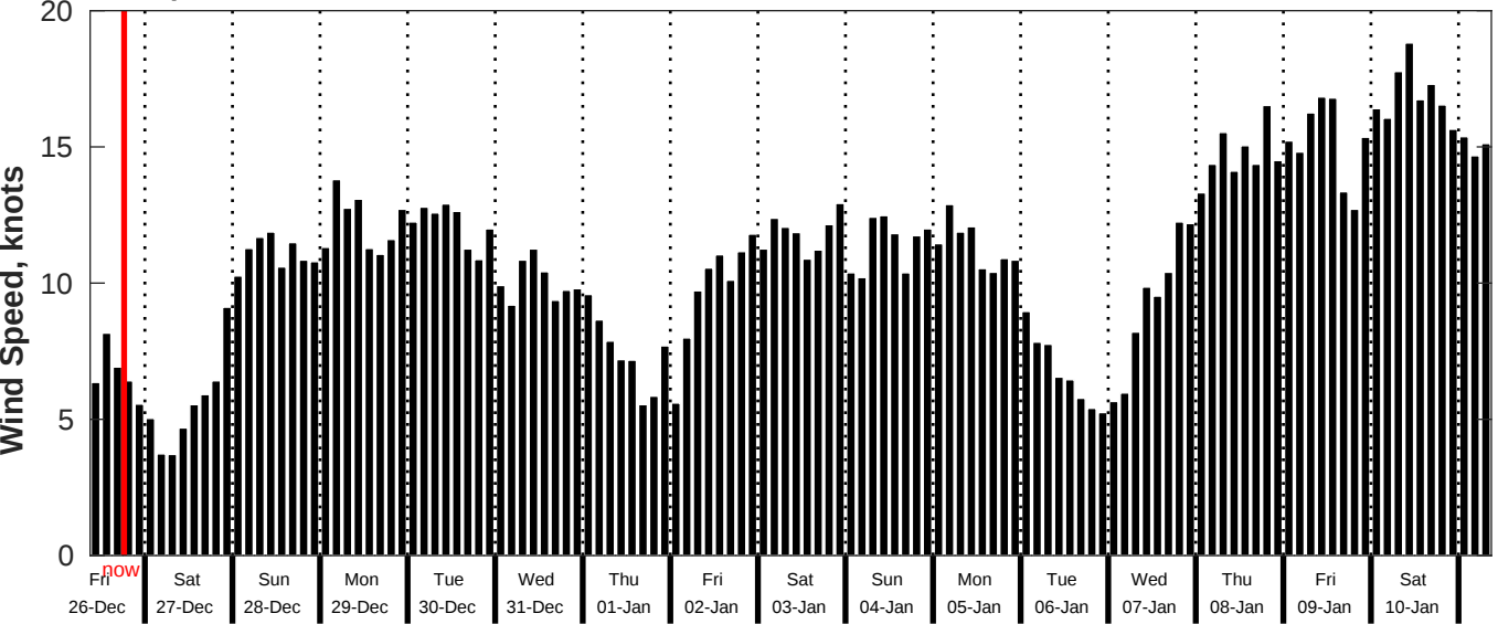
GFS Wind Speed Forecast for NDBC 52212 from 25-Dec-2025 09:00:00 to 10-Jan-2026 09:00:00
