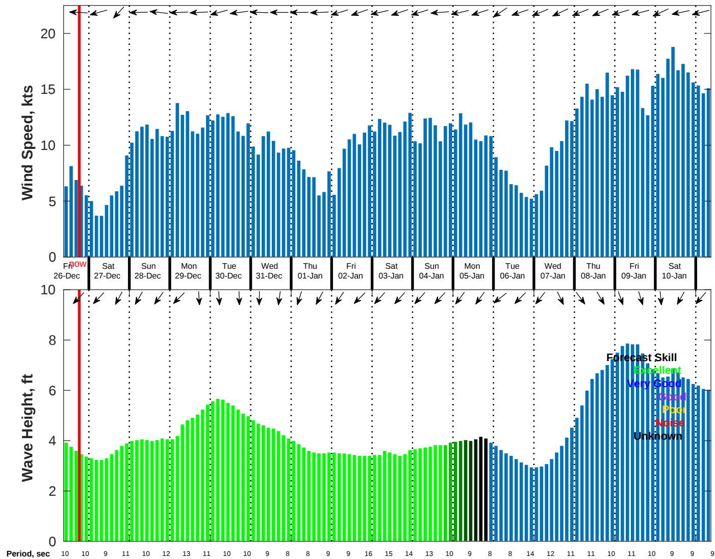
Wind & Wave Forecast for NDBC 52212 from 25-Dec-2025 09:00:00 to 10-Jan-2026 09:00:00
