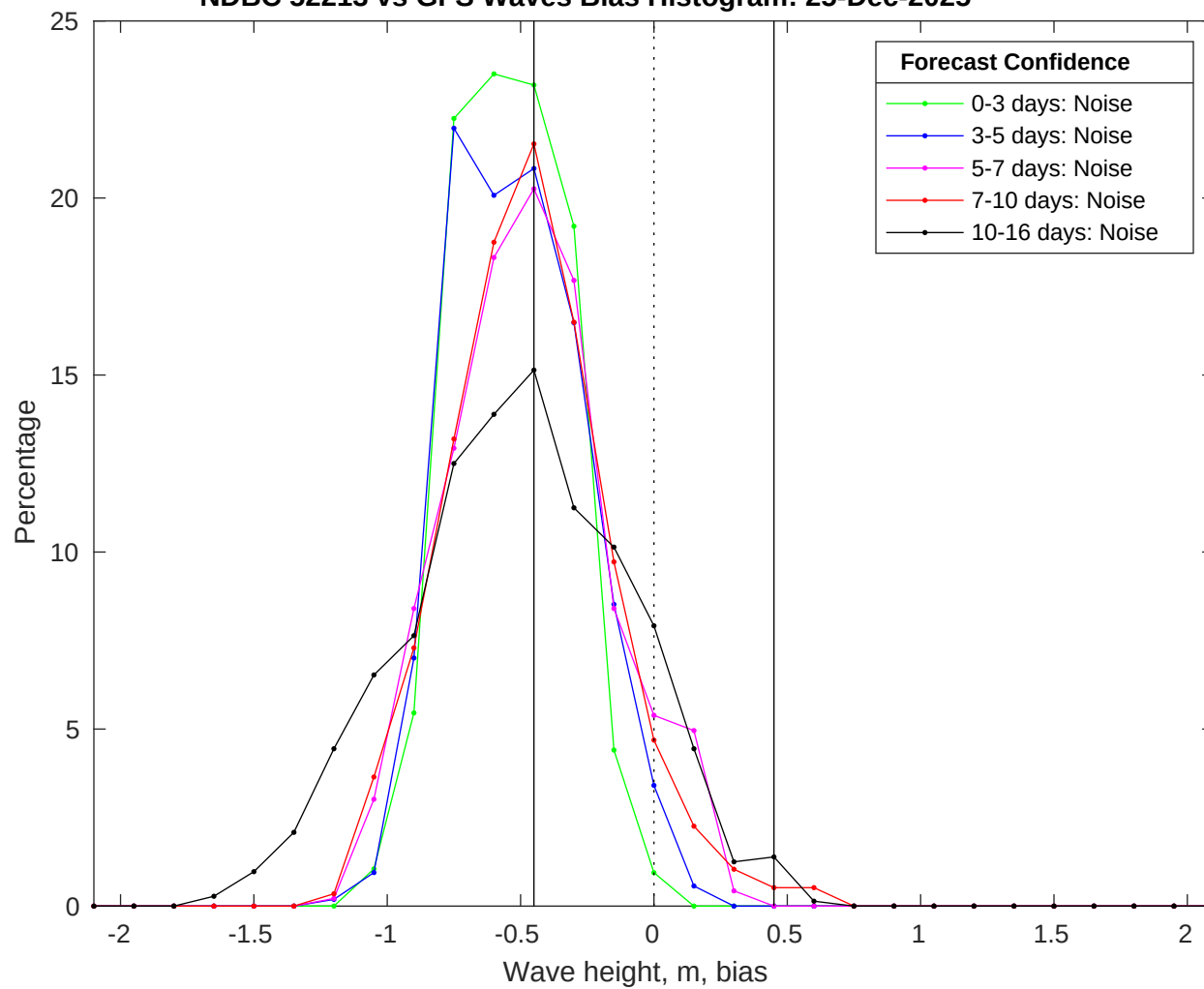
NDBC 52213 vs GFS Waves Bias Histogram: 25-Dec-2025
