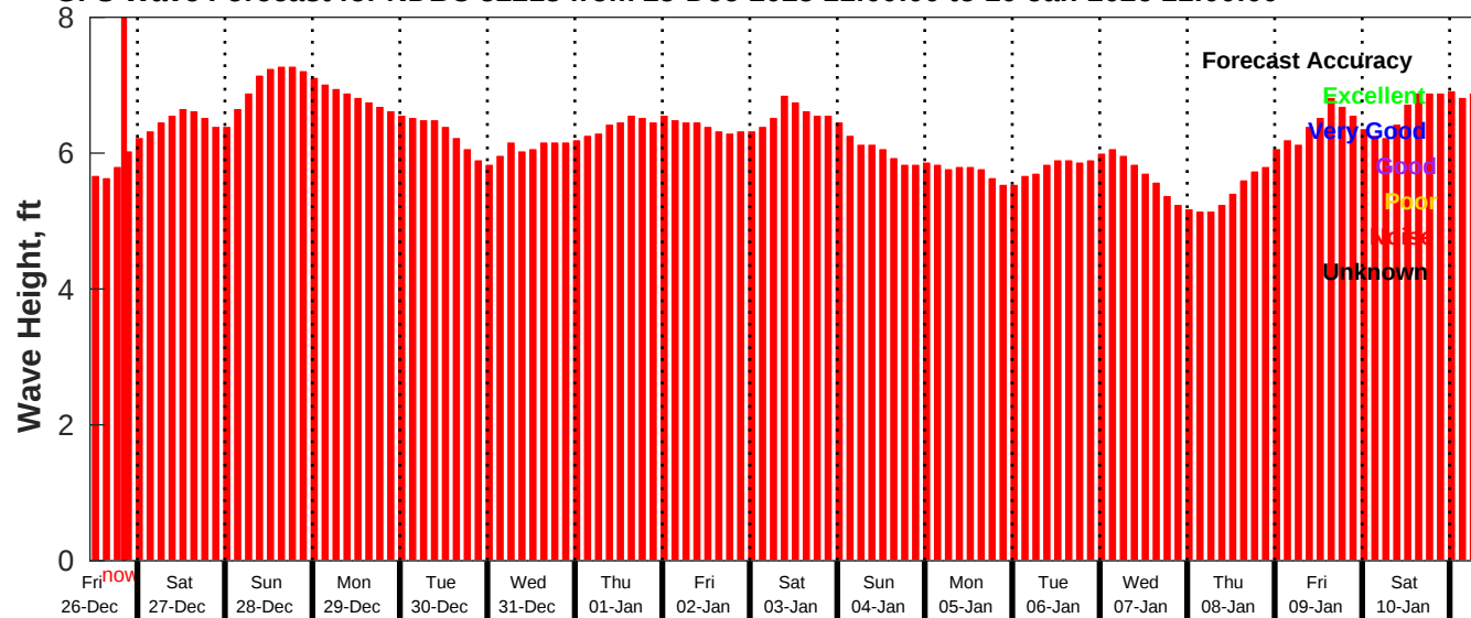
GFS Wave Forecast for NDBC 52213 from 25-Dec-2025 11:00:00 to 10-Jan-2026 11:00:00
