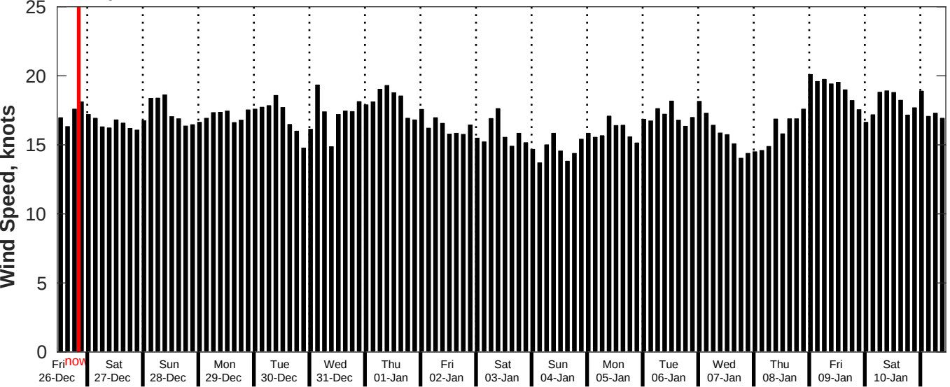
GFS Wind Speed Forecast for NDBC 52213 from 25-Dec-2025 11:00:00 to 10-Jan-2026 11:00:00
