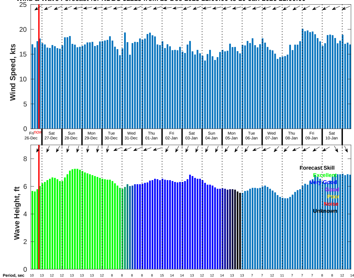
Wind & Wave Forecast for NDBC 52213 from 25-Dec-2025 11:00:00 to 10-Jan-2026 11:00:00
