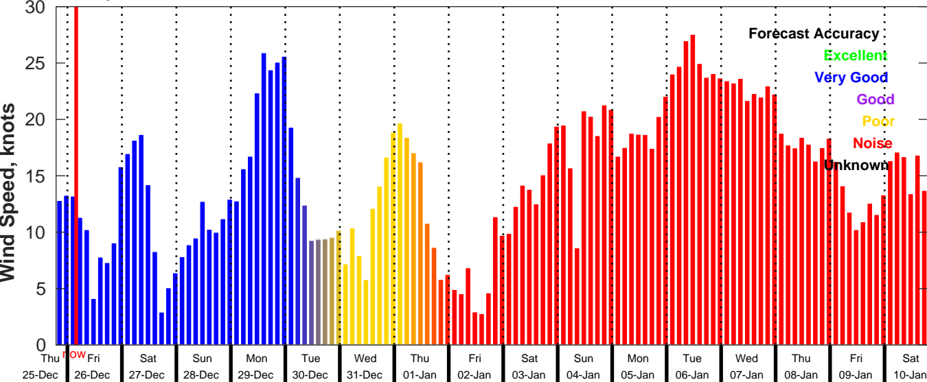
GFS Wind Speed Forecast for NDBC 41004 from 25-Dec-2025 19:00:00 to 10-Jan-2026 19:00:00
