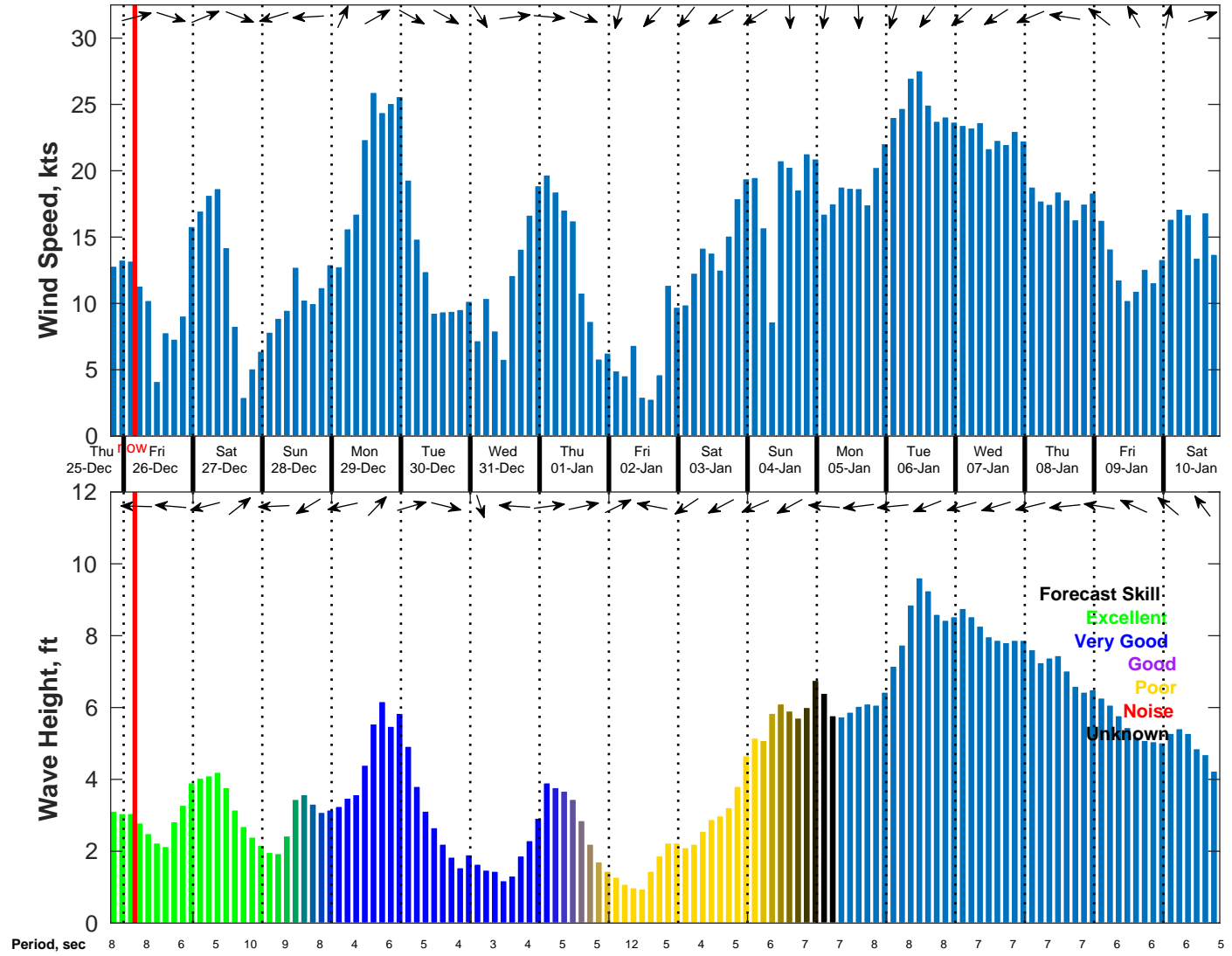
Wind & Wave Forecast for NDBC 41004 from 25-Dec-2025 19:00:00 to 10-Jan-2026 19:00:00
