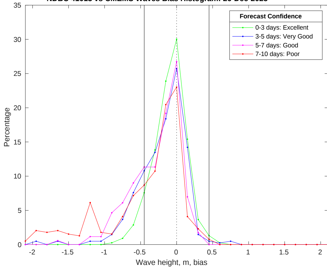
NDBC 41013 vs CMEMS Waves Bias Histogram: 26-Dec-2025
