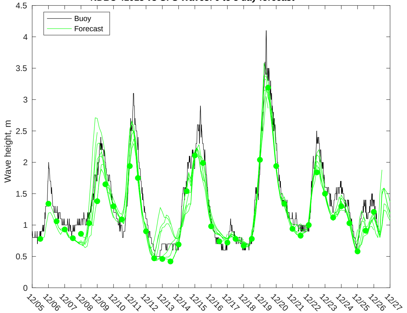
NDBC 41013 vs GFS Waves: 0 to 3 day forecast
