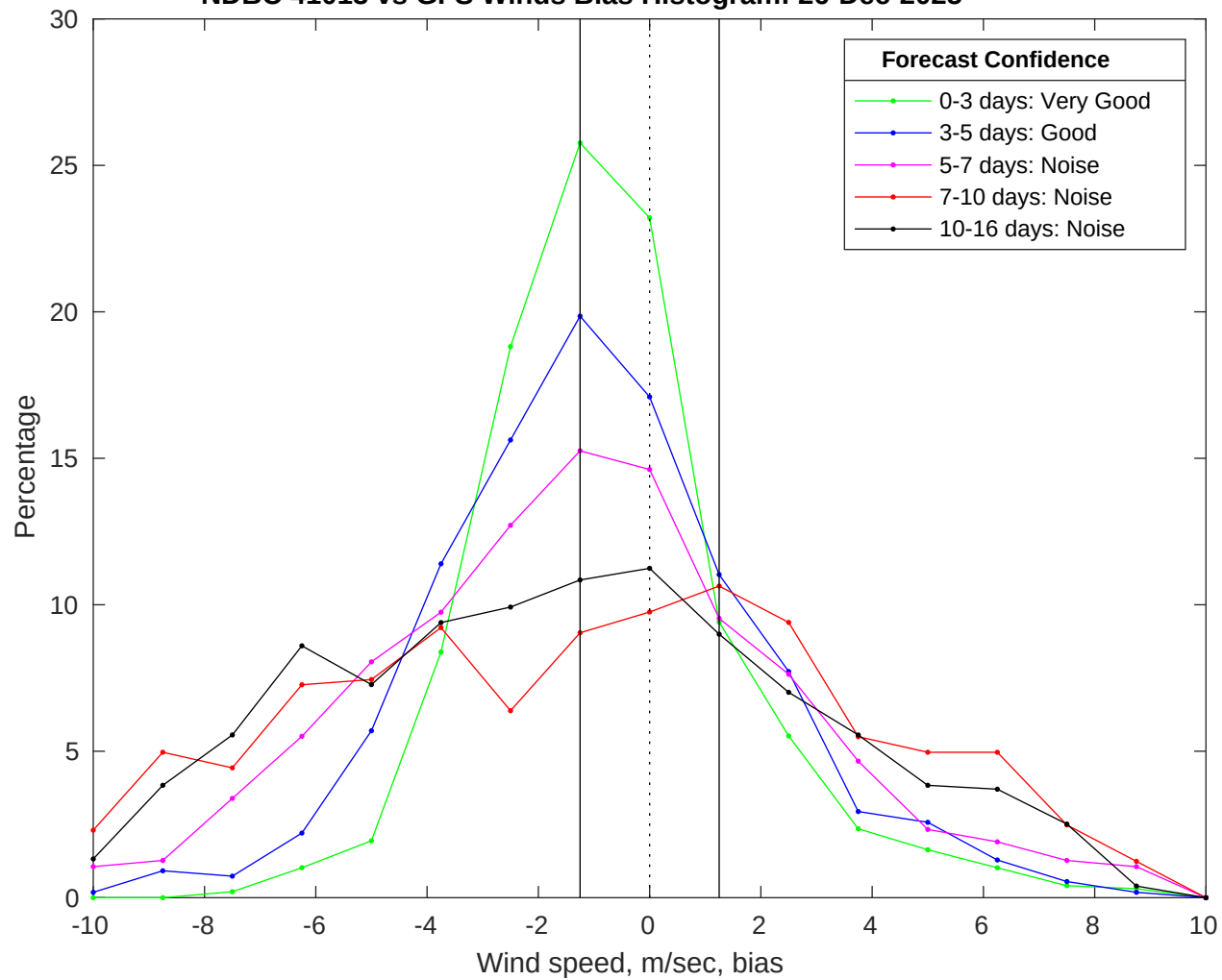
NDBC 41013 vs GFS Winds Bias Histogram: 26-Dec-2025
