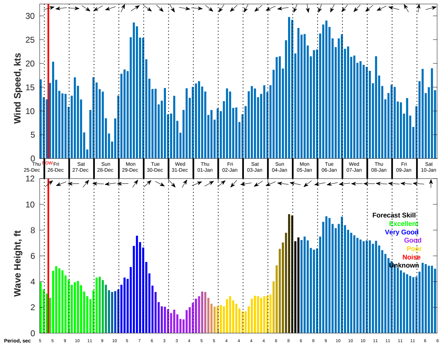
Wind & Wave Forecast for NDBC 41013 from 25-Dec-2025 19:00:00 to 10-Jan-2026 19:00:00
