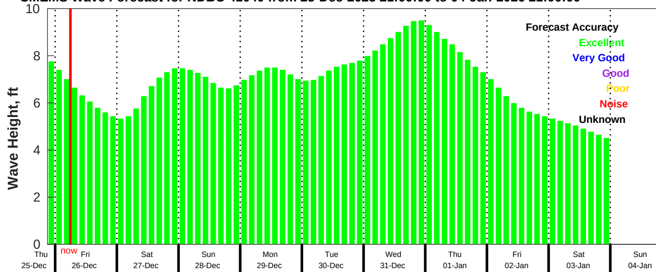
CMEMS Wave Forecast for NDBC 41040 from 25-Dec-2025 21:00:00 to 04-Jan-2026 21:00:00
