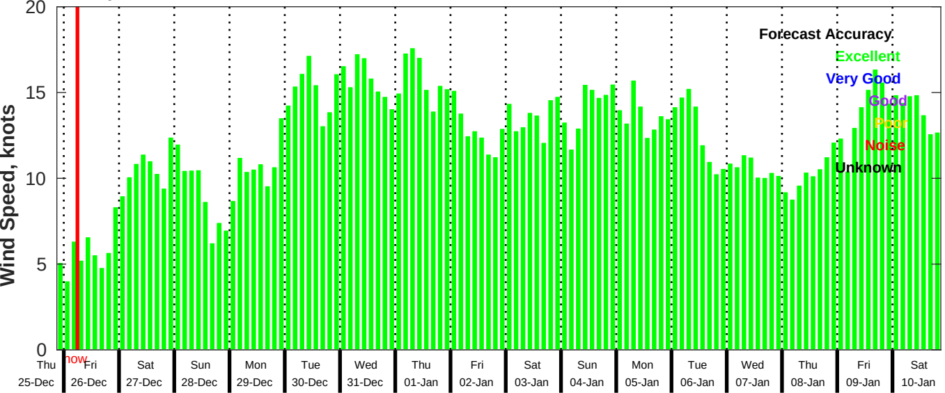
GFS Wind Speed Forecast for NDBC 41040 from 25-Dec-2025 21:00:00 to 10-Jan-2026 21:00:00
