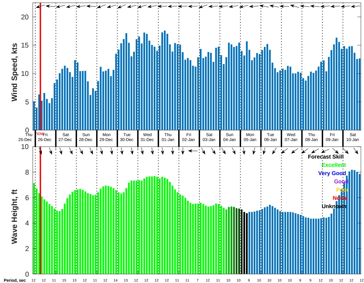
Wind & Wave Forecast for NDBC 41040 from 25-Dec-2025 21:00:00 to 10-Jan-2026 21:00:00
