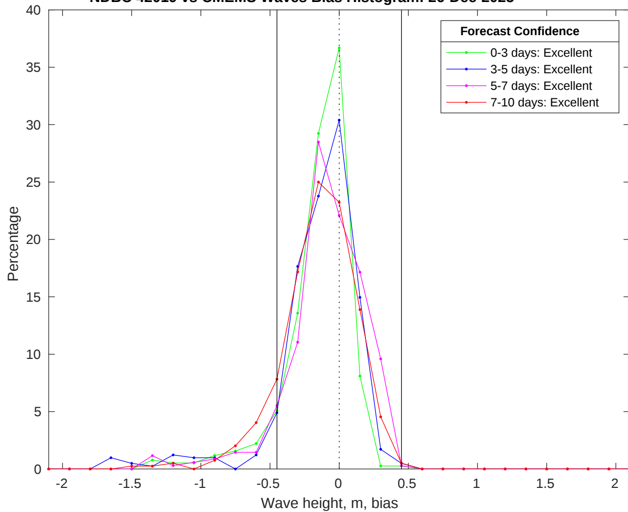
NDBC 42019 vs CMEMS Waves Bias Histogram: 26-Dec-2025
