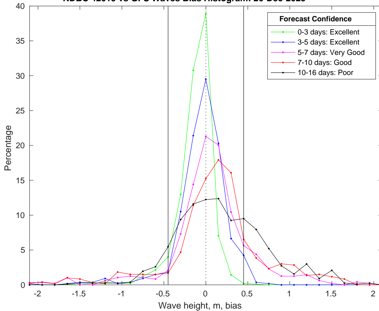
NDBC 42019 vs GFS Waves Bias Histogram: 26-Dec-2025
