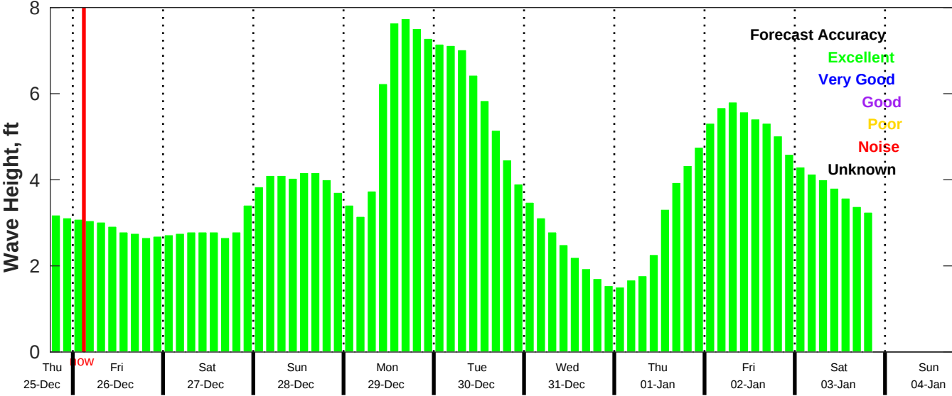
CMEMS Wave Forecast for NDBC 42019 from 25-Dec-2025 18:00:00 to 04-Jan-2026 18:00:00
