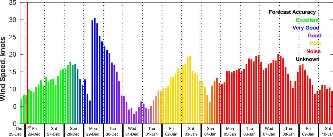
GFS Wind Speed Forecast for NDBC 42019 from 25-Dec-2025 18:00:00 to 10-Jan-2026 18:00:00
