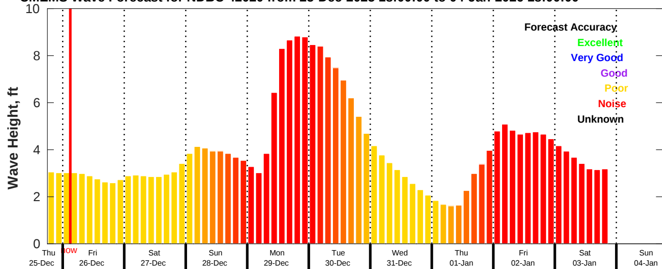
CMEMS Wave Forecast for NDBC 42020 from 25-Dec-2025 18:00:00 to 04-Jan-2026 18:00:00
