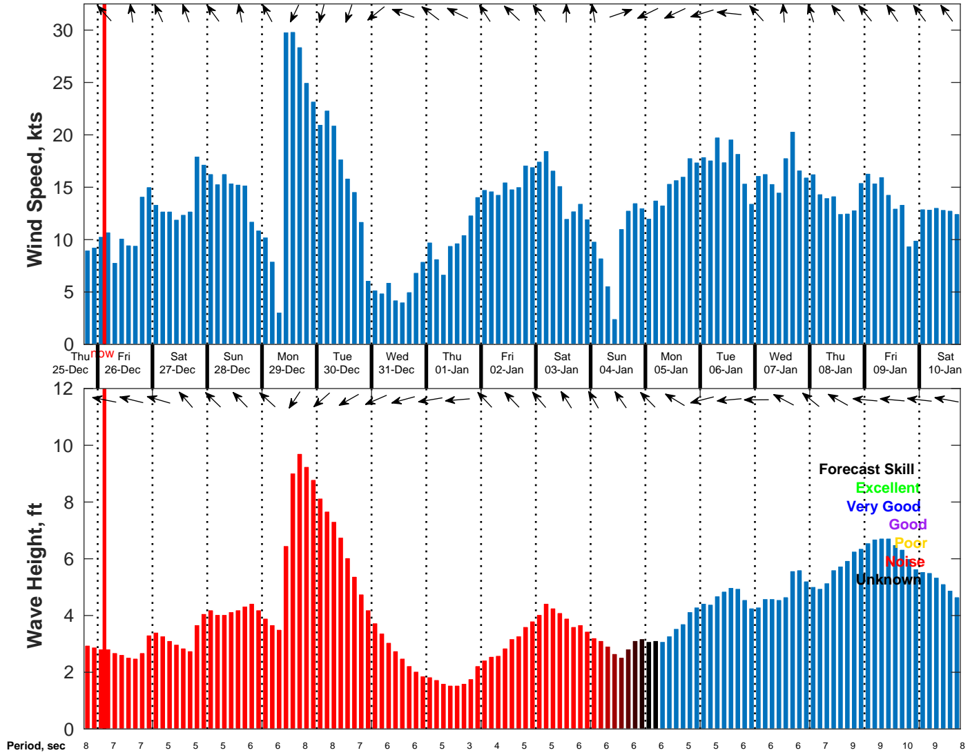
Wind & Wave Forecast for NDBC 42020 from 25-Dec-2025 18:00:00 to 10-Jan-2026 18:00:00
