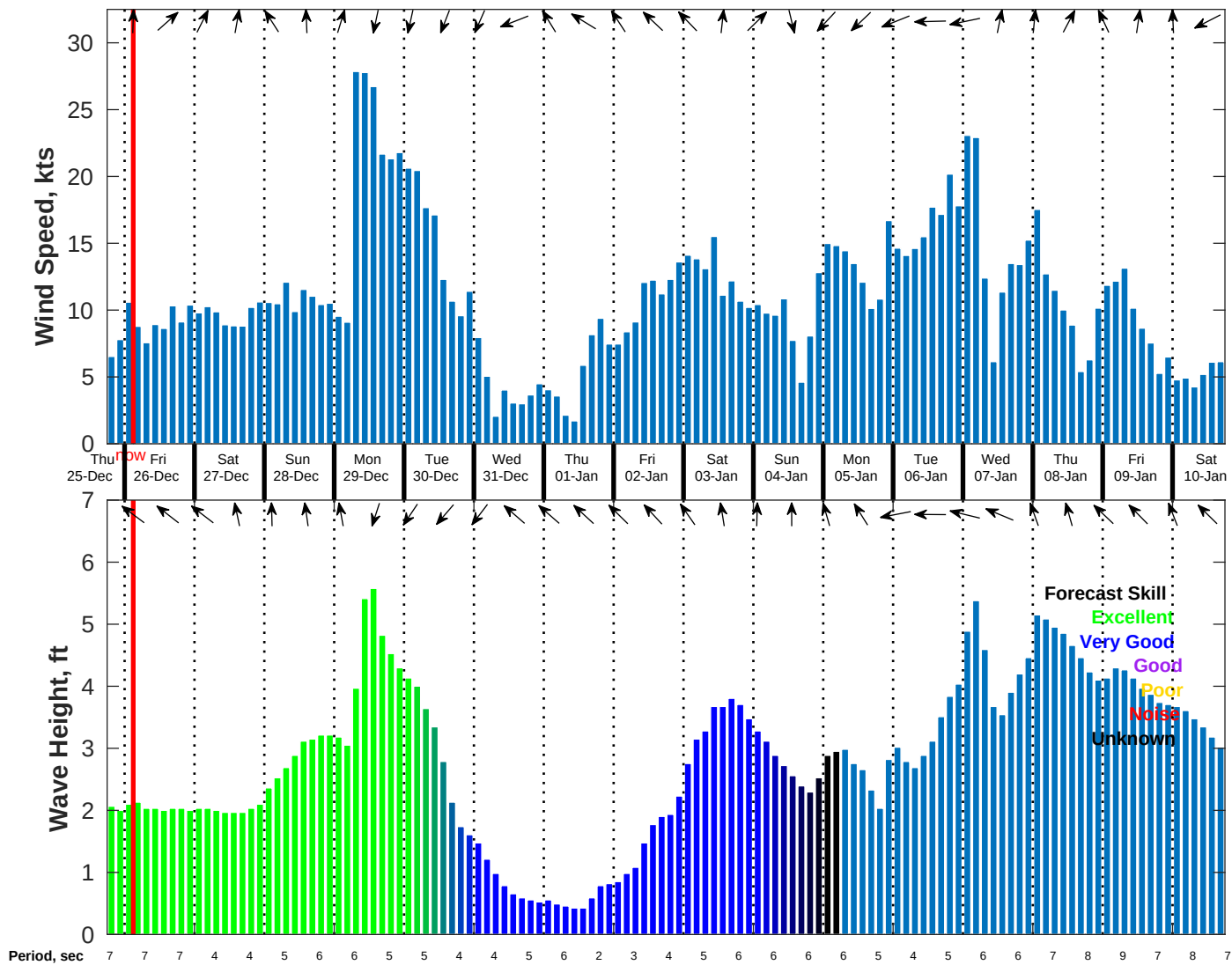
Wind & Wave Forecast for NDBC 42035 from 25-Dec-2025 18:00:00 to 10-Jan-2026 18:00:00
