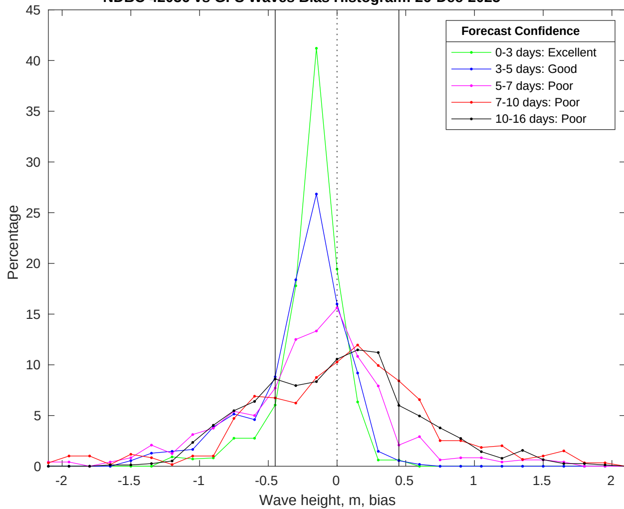
NDBC 42036 vs GFS Waves Bias Histogram: 26-Dec-2025
