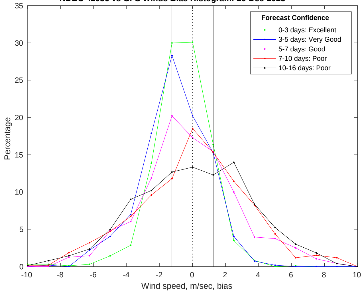
NDBC 42036 vs GFS Winds Bias Histogram: 26-Dec-2025
