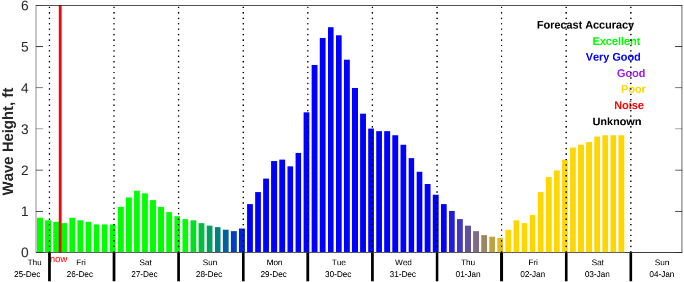
CMEMS Wave Forecast for NDBC 42036 from 25-Dec-2025 19:00:00 to 04-Jan-2026 19:00:00
