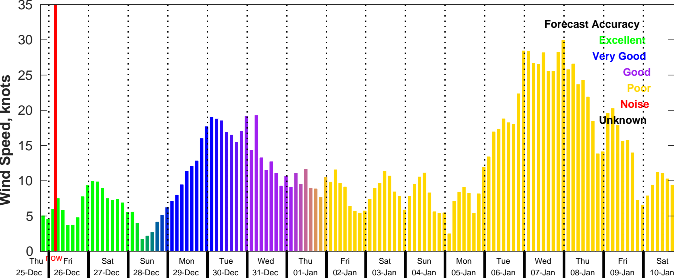
GFS Wind Speed Forecast for NDBC 42036 from 25-Dec-2025 19:00:00 to 10-Jan-2026 19:00:00
