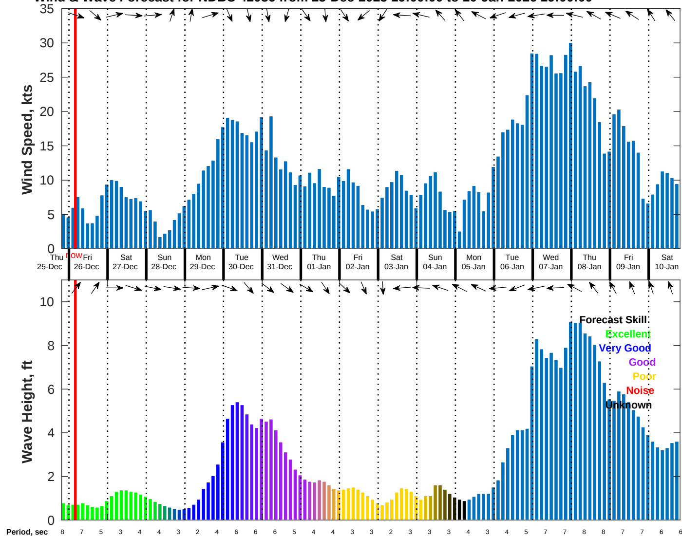
Wind & Wave Forecast for NDBC 42036 from 25-Dec-2025 19:00:00 to 10-Jan-2026 19:00:00
