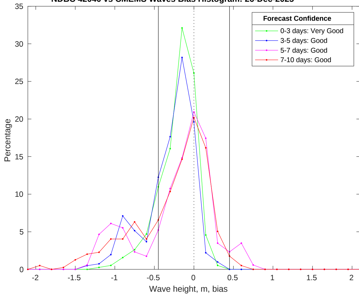
NDBC 42040 vs CMEMS Waves Bias Histogram: 26-Dec-2025
