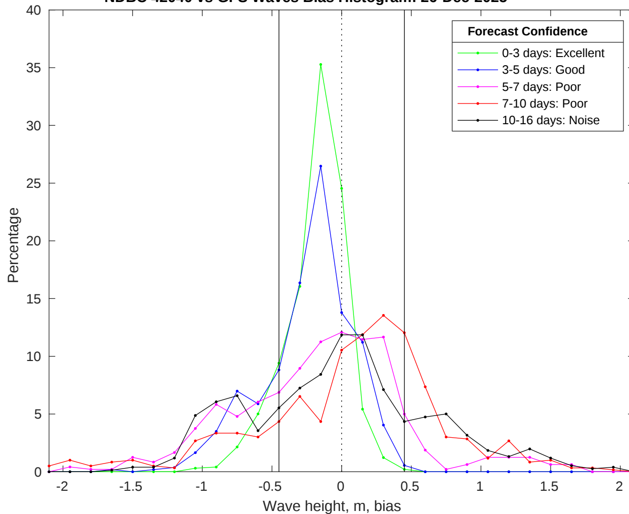
NDBC 42040 vs GFS Waves Bias Histogram: 26-Dec-2025
