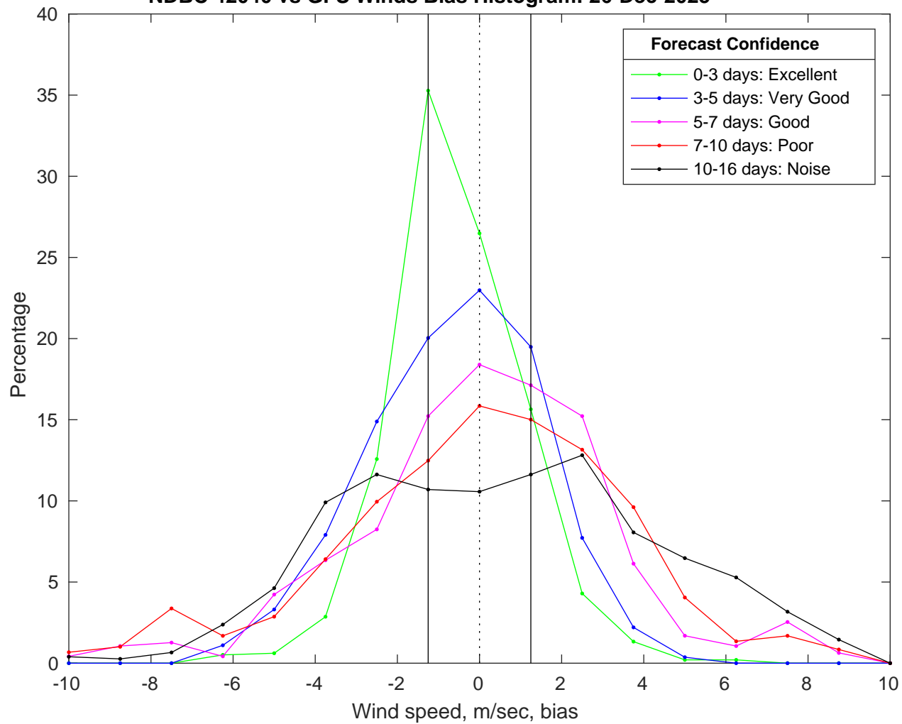
NDBC 42040 vs GFS Winds Bias Histogram: 26-Dec-2025
